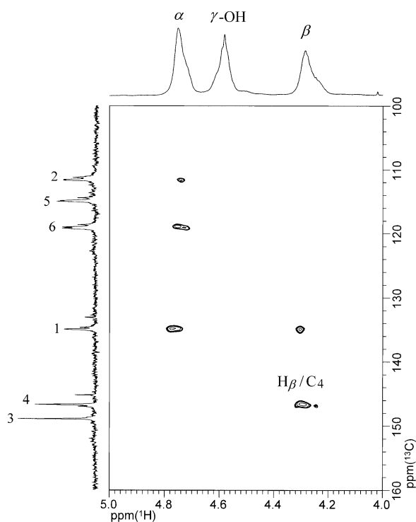
Fig. 6 HMBC spectrum of \beta -O-4 type artificial lignin polymer 2 in DMSO- d_6 .
