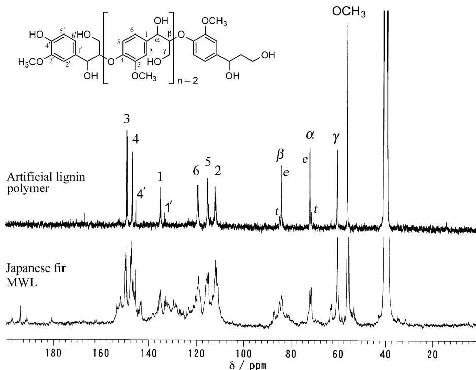
Fig. 3 13 C-NMR spectra of \beta -O-4 type artificial lignin polymer 2 and Japanese fir MWL. 1',4': phenolic end units; e: erythro, t: threo; MWL: milled wood lignin. The structure of non-phenolic end units is uncertain.
